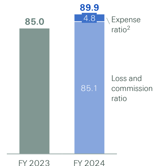
Combined ratio 1 (%)
